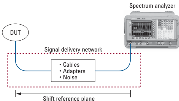
Figure 6. Test setup
